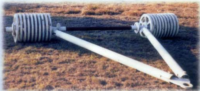
Disc rollers
